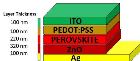
Fig. 16. Simulated Perovskite Solar cell with layer Thickness
