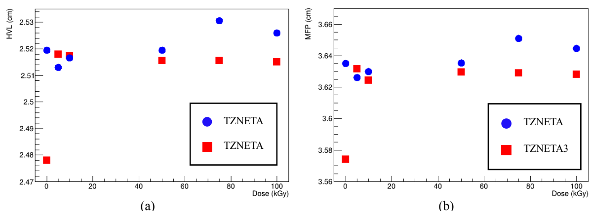
Fig. 5. Graph of a) HVL and b) MFP TZNETA3 and TZNETA6 pre- and post-irradiation
